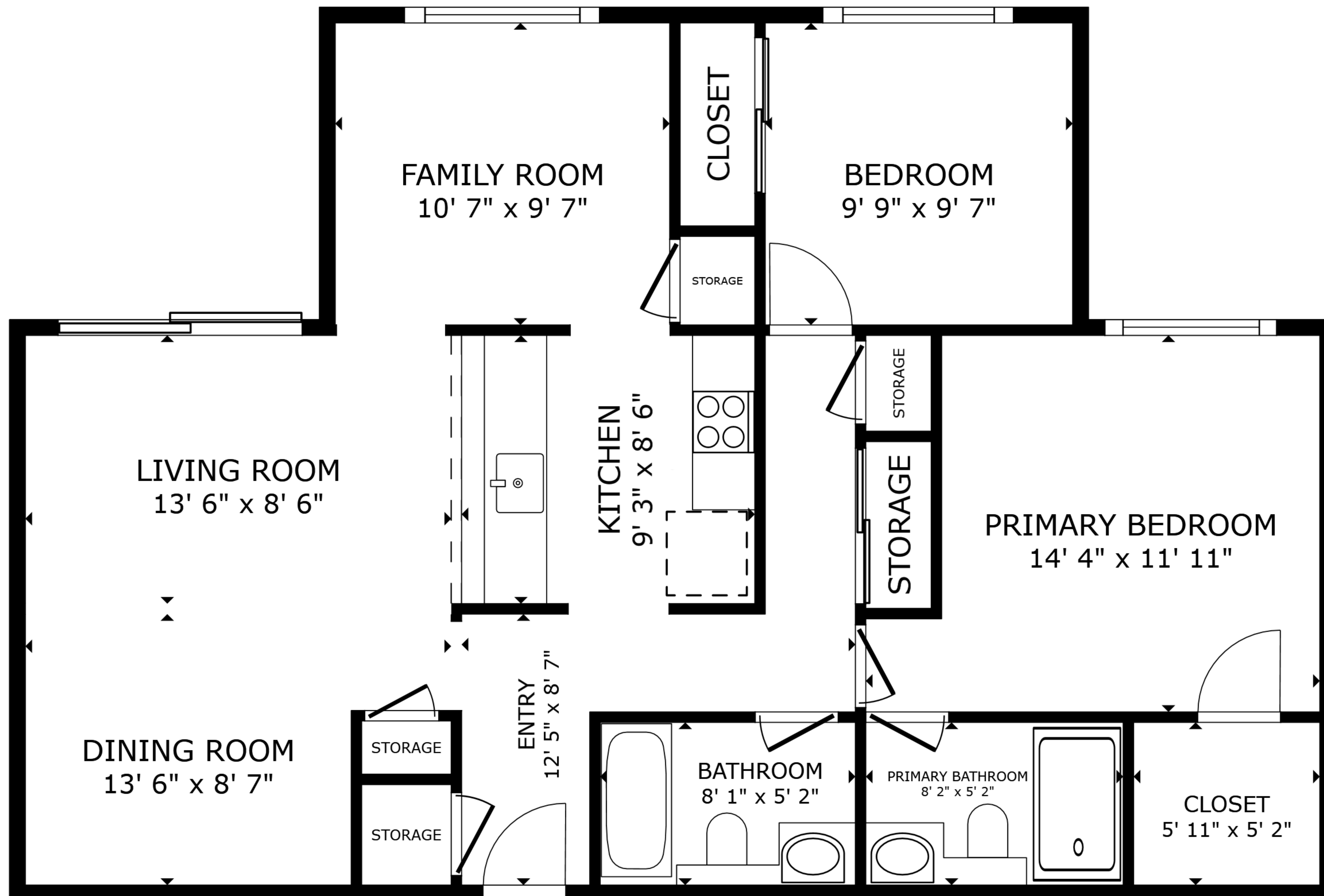
FLOOR PLAN
