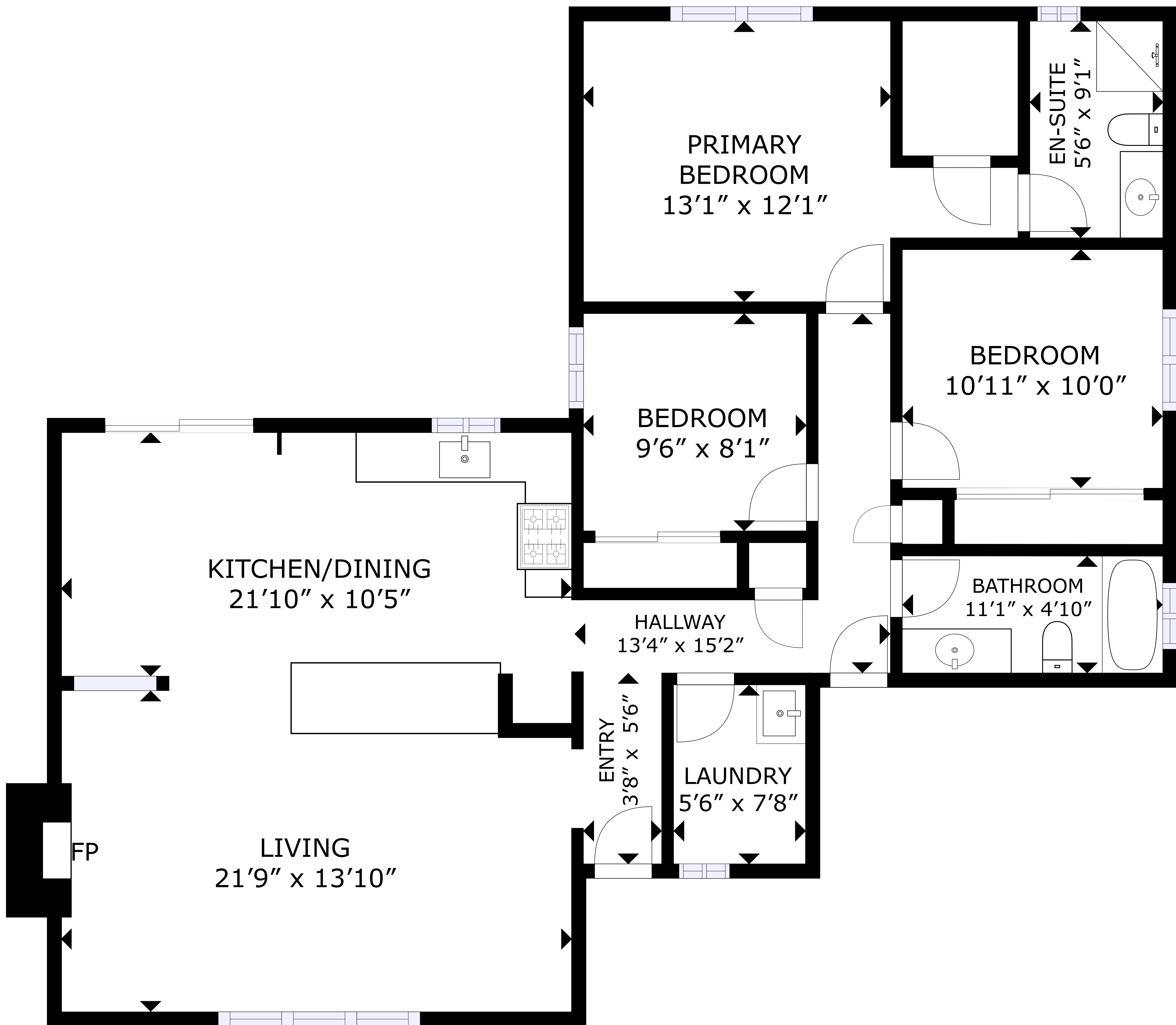
FLOOR PLAN
