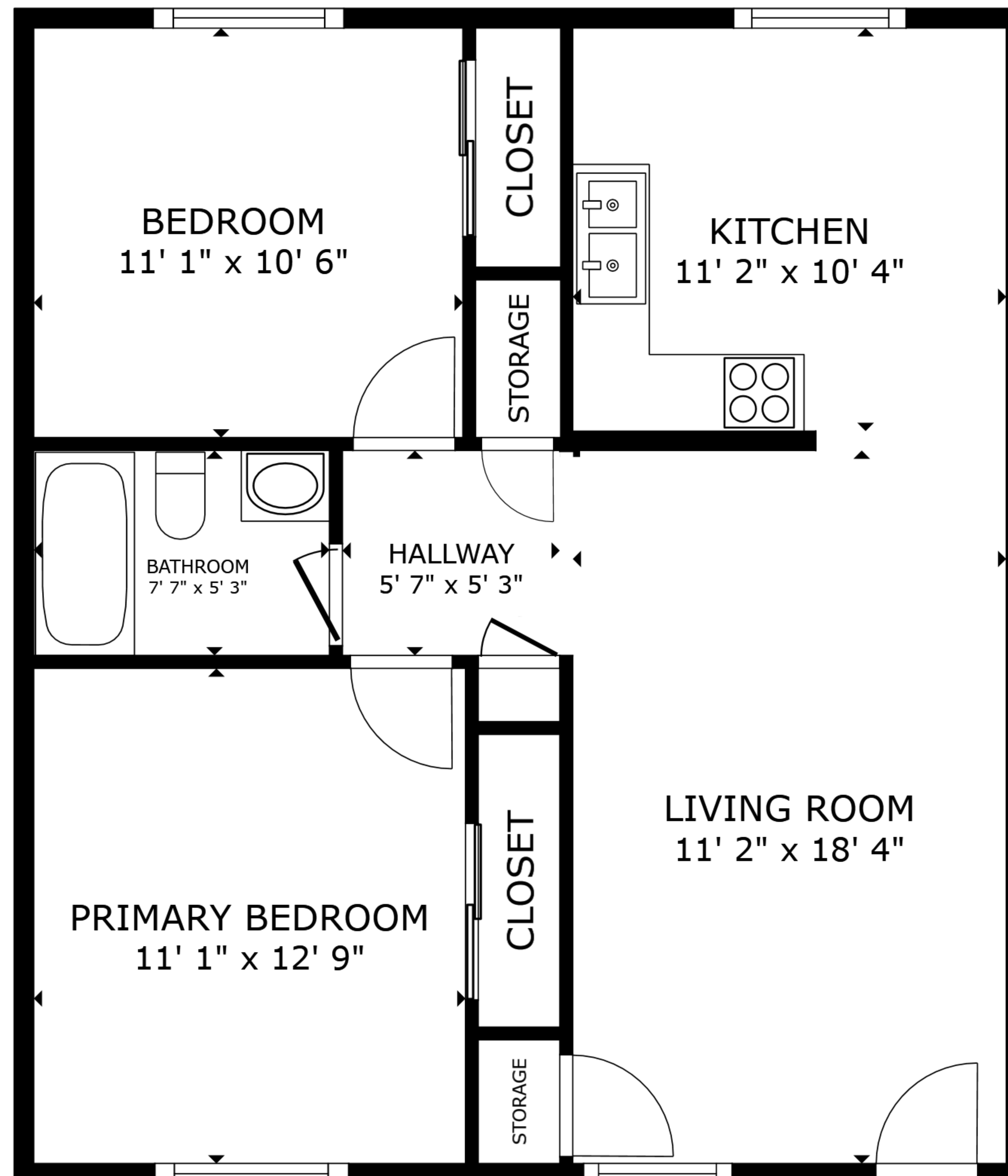
FLOOR PLAN
