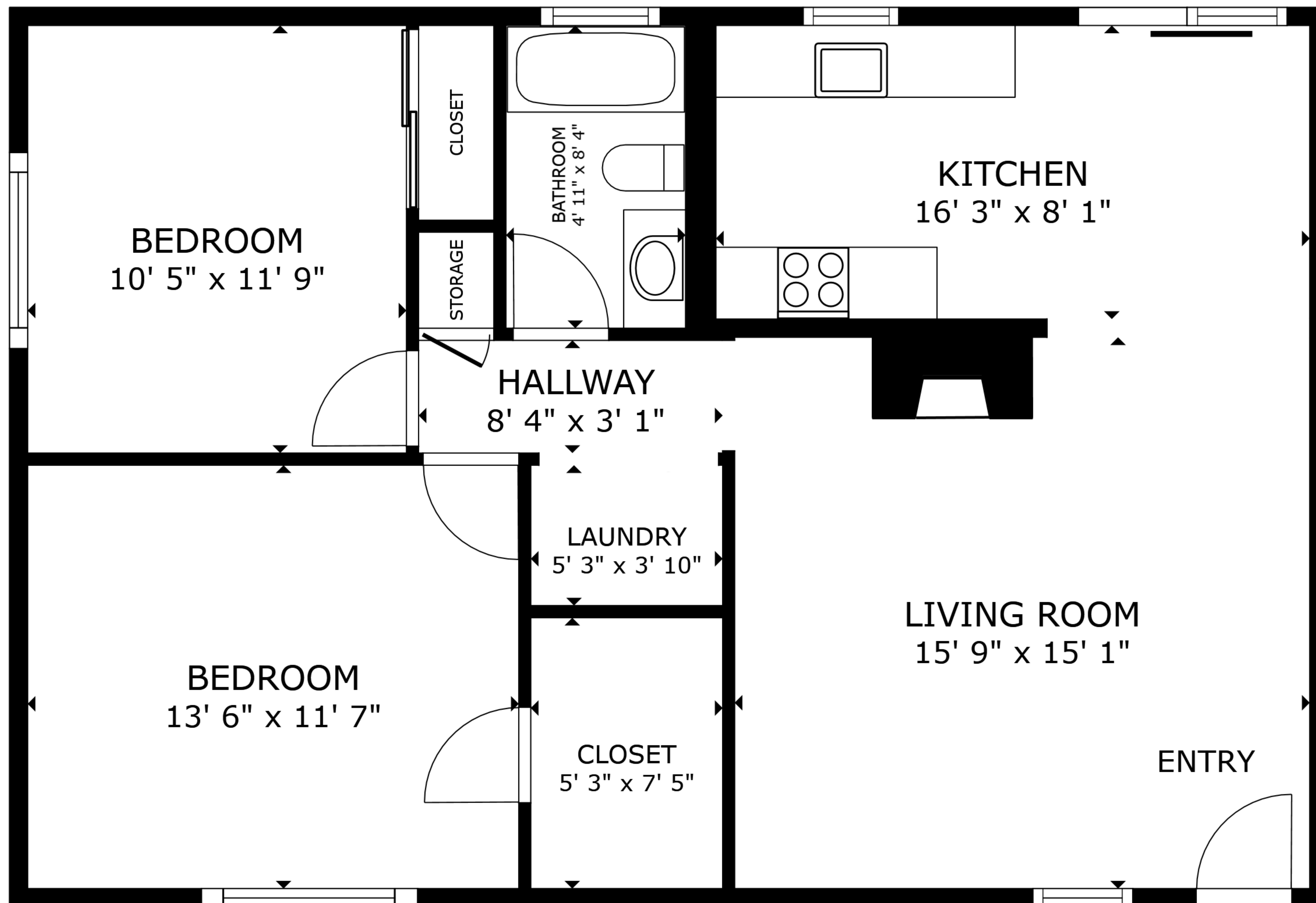
FLOOR PLAN
